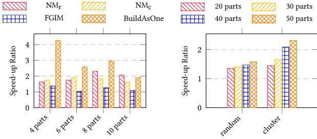
Figure 10: Speed-up Ratio Comparison across Different Partitions with MARCO10M
