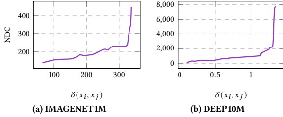
Figure 5: Verification of Distance Cost Model. In datasets IMAGENET1M and DEEP10M, the cost of sliding from x_i to x_j is linear to the distance when x_i and x_j are close[65].
