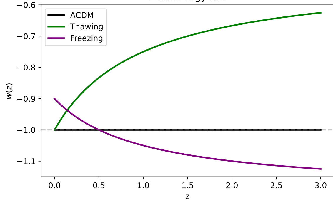
Dark Energy EoS
