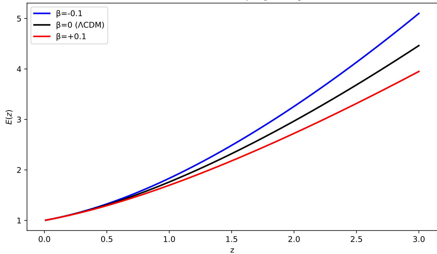
ILCDM: Different Coupling Strengths
