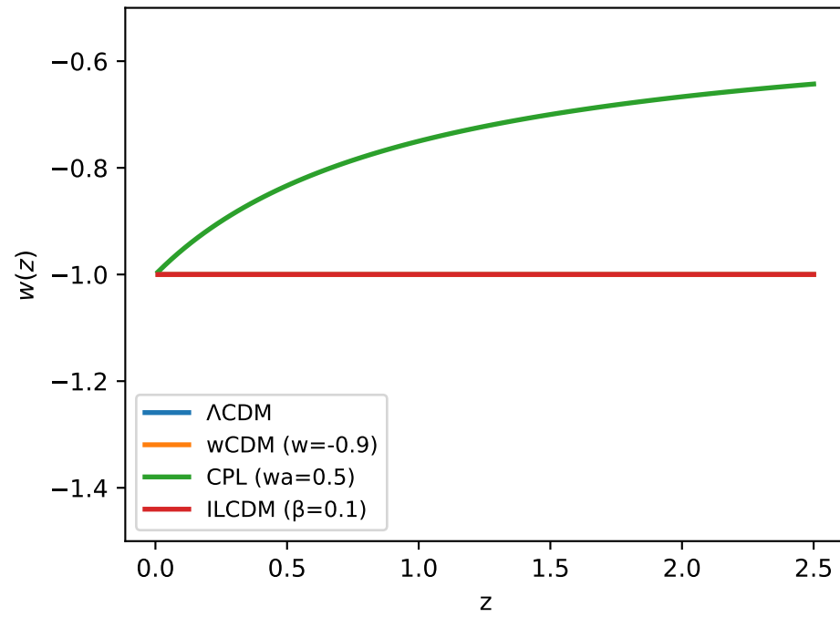
Dark Energy EoS
