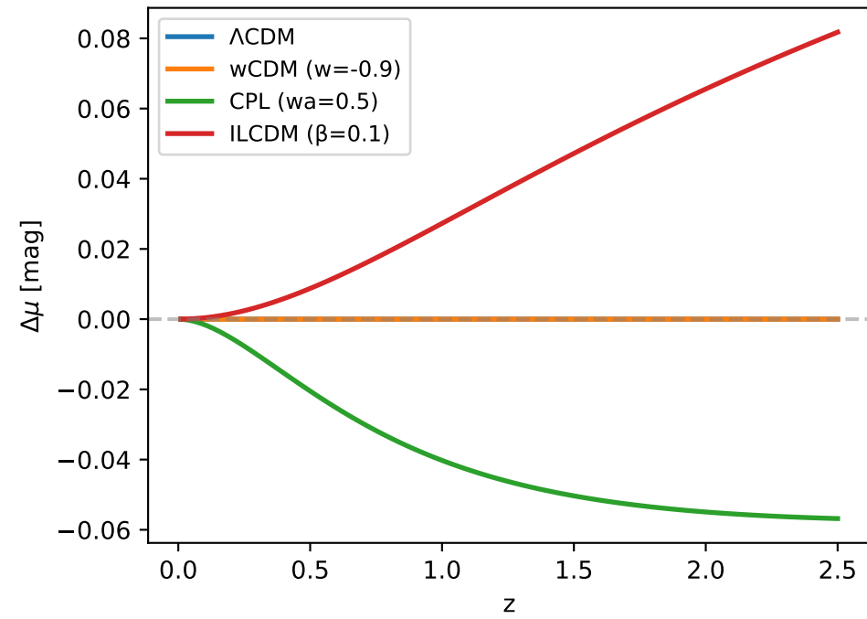
Distance Modulus (compare to \Lambda CDM)
