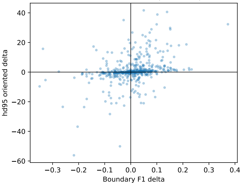
acdc: BF1 vs hd95 (rho=0.56)
