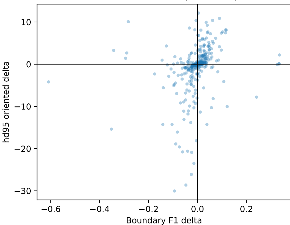
synapse: BF1 vs hd95 (rho=0.24)
