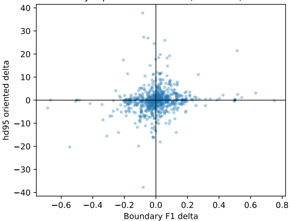
synapse: BF1 vs hd95 (rho=0.24)
