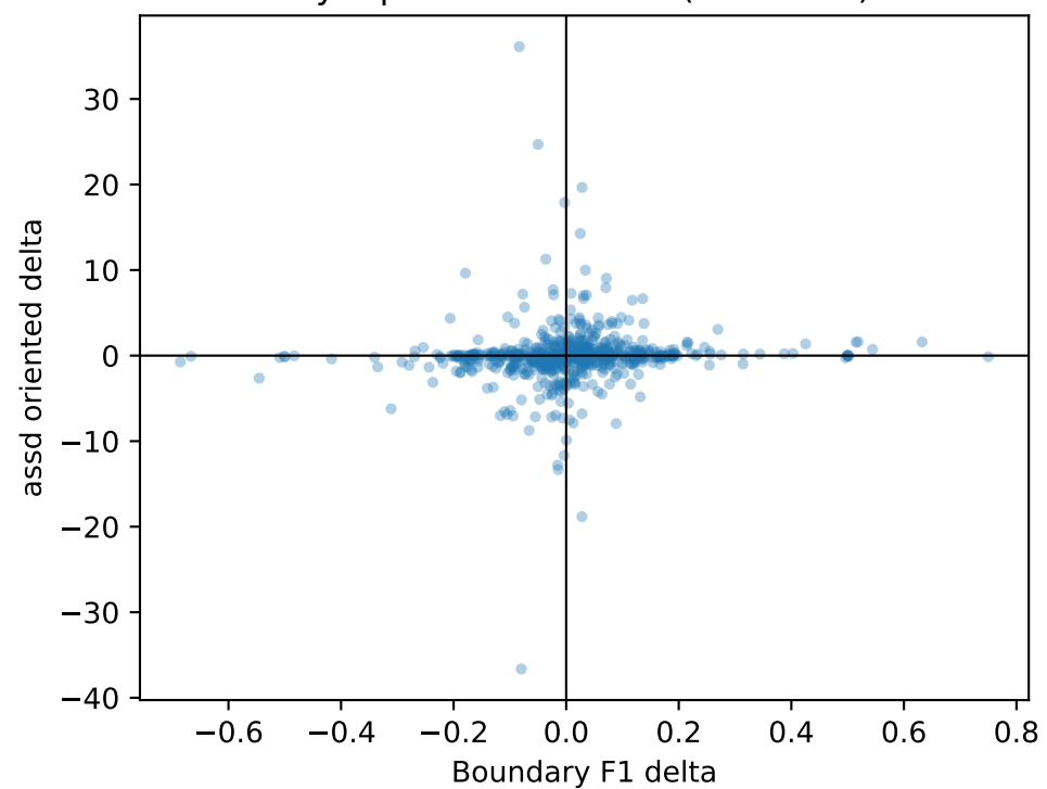
synapse: BF1 vs asdd (rho=0.25)
