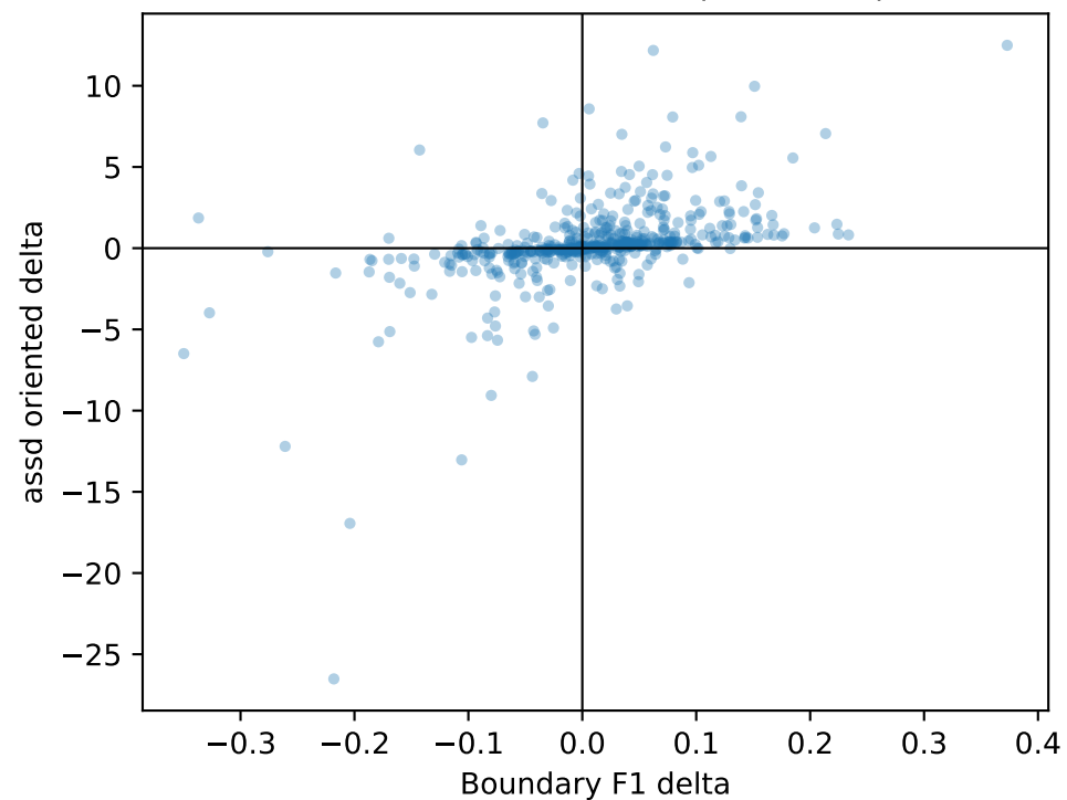
acdc: BF1 vs asdd (rho=0.62)
