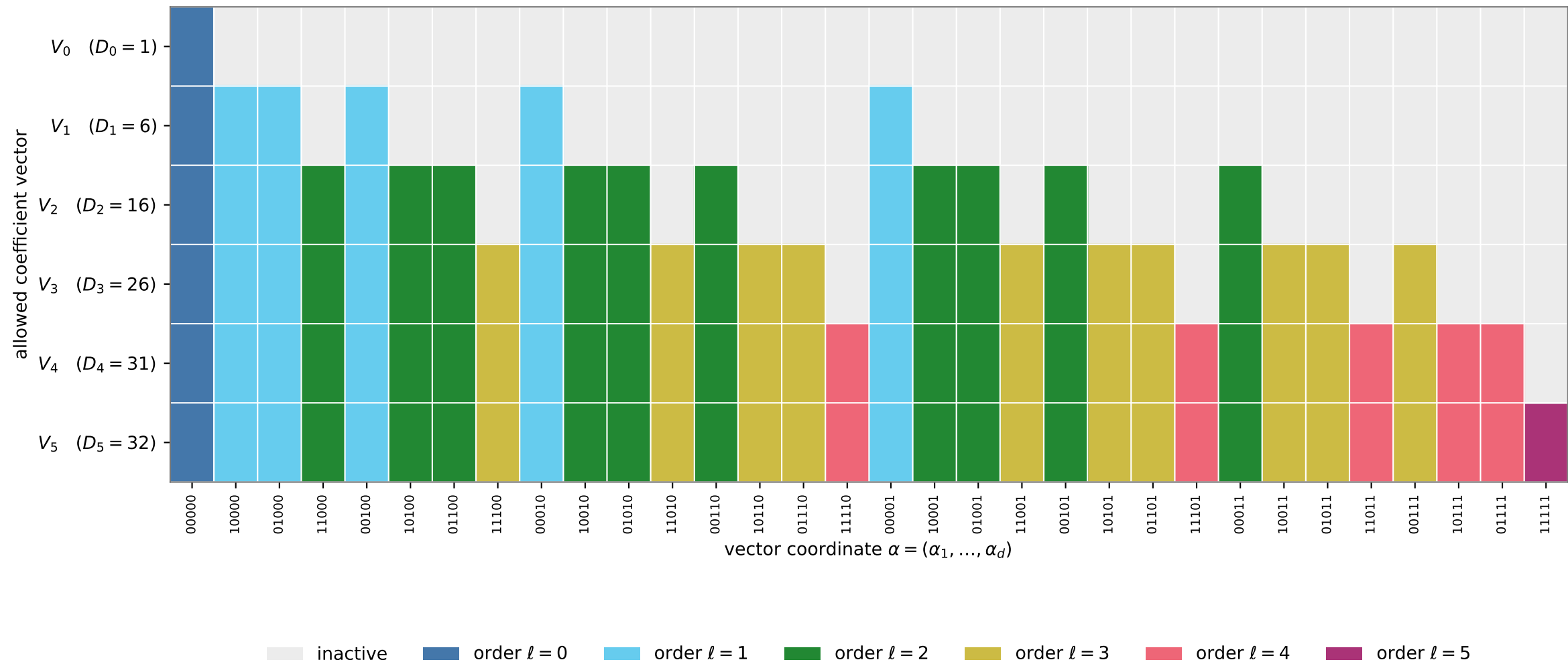
Growth of V_s for a binary tensor with d = 5 ( N = 2^d = 32 )
