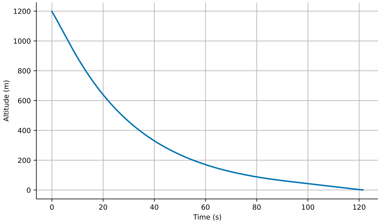
Powered descent feedback control
