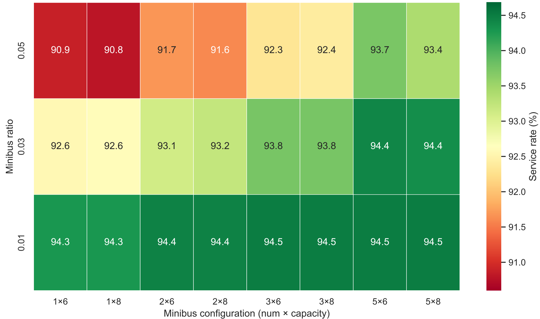
Service rate under the time-optimal policy
