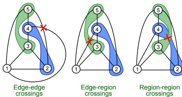
Figure 17.1: C-planar crossings
