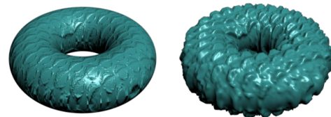
Bump Mapping
