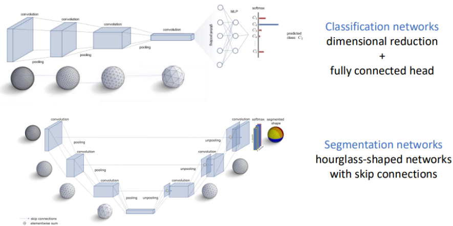
Figure 19.1: Network architectures
