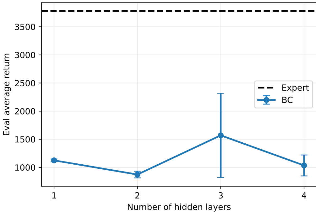
BC Hyperparameter Sweep on Hopper-v2
