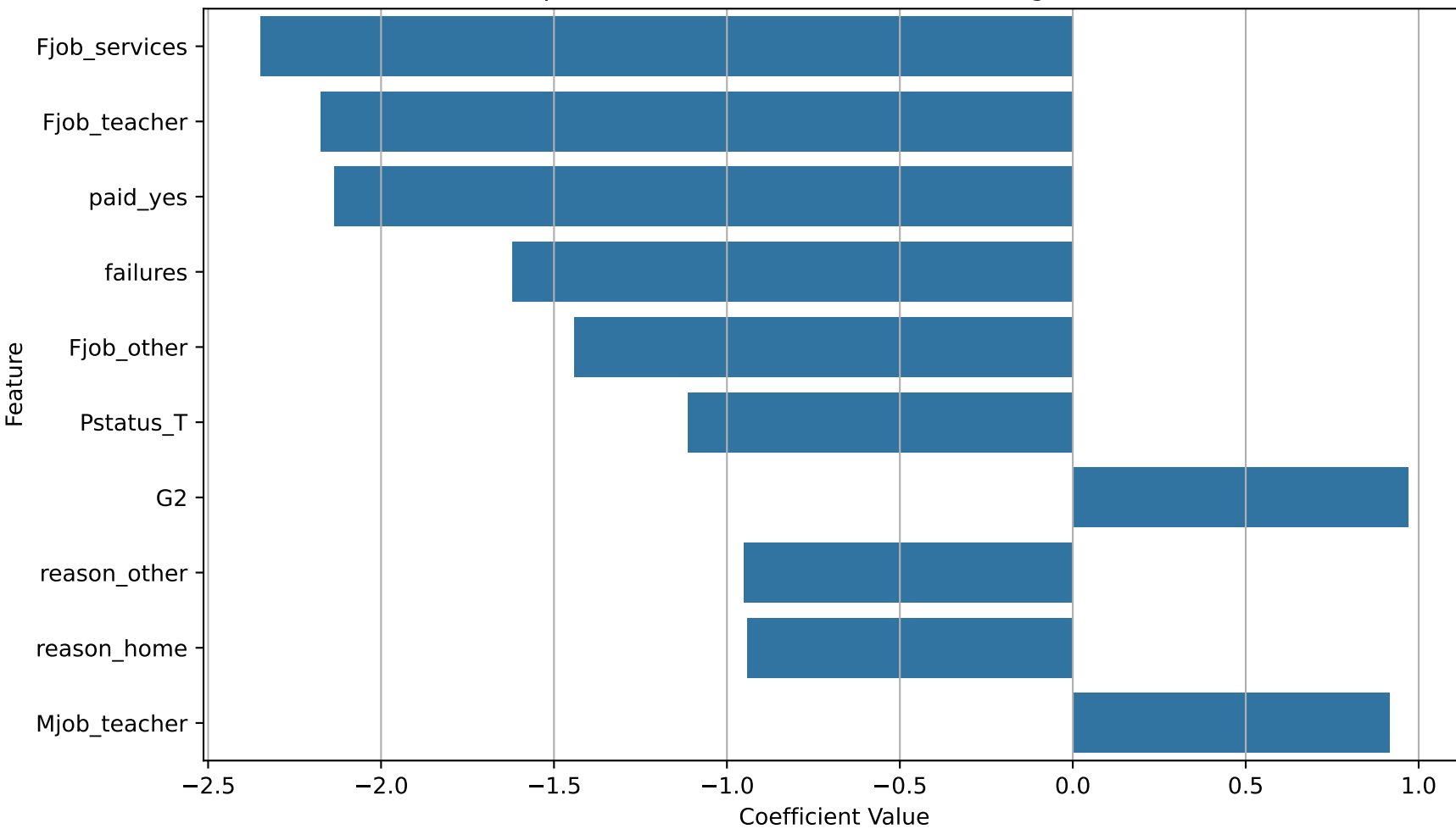
Top 10 Feature Coefficients (Linear Regression)
