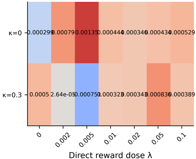
confounded
