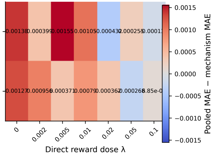
independent latents
