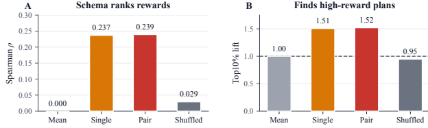
Figure 5: Schema-space reward predictability.
