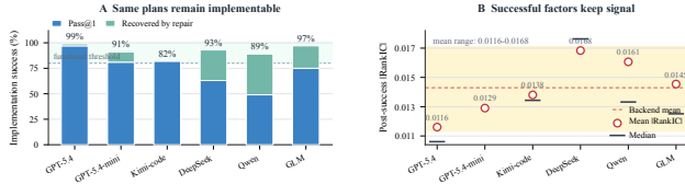
Figure 4: Repair-aware robustness to code-agent backends on the same 100 schema plans. Panel A separates first-attempt implementation success from repair recovery; Panel B shows that successful implementations retain comparable signal quality across backends.
