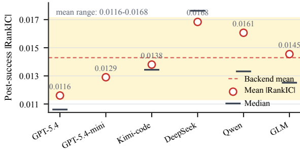
B Successful factors keep signal
