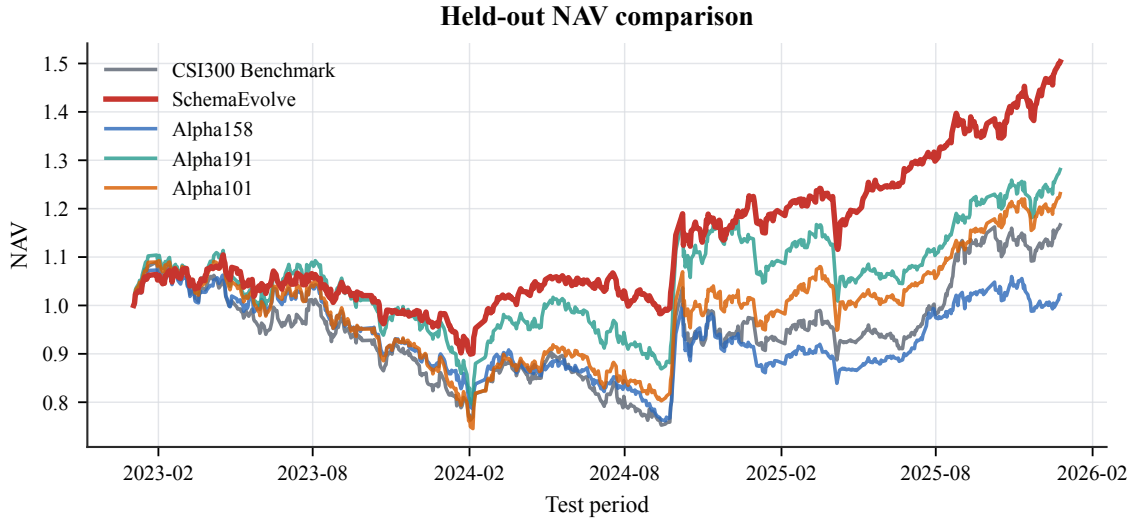
Figure 2: Held-out NAV comparison against representative open-source factor libraries on CSI300 over the 2023–2025 test period. All curves are evaluated under the same CSRankNorm, LightGBM combiner, and Top50/Drop5 backtest protocol.
