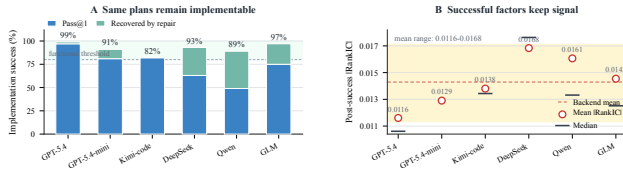
Figure 3: Repair-aware robustness to code-agent backends on the same 100 schema plans. Panel A separates first-attempt implementation success from repair recovery; Panel B shows that successful implementations retain comparable signal quality across backends.
