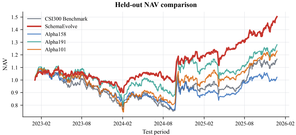
Figure 1: Held-out NAV comparison against representative open-source factor libraries on CSI300 over the 2023–2025 test period. All curves are evaluated under the same CSRankNorm, LightGBM combiner, and Top50/Drop5 backtest protocol.
