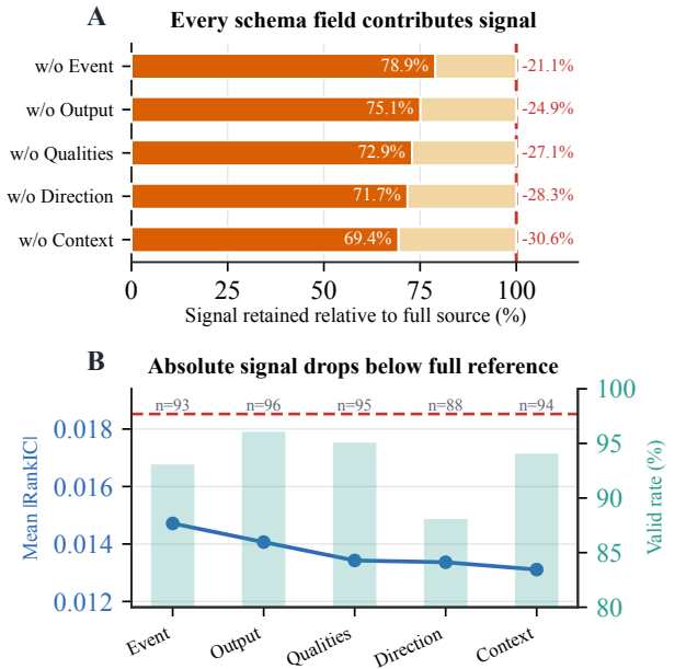
Figure 3: Component-wise schema ablation.
