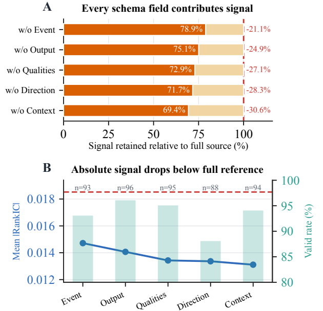
Figure 3: Component-wise schema ablation.
