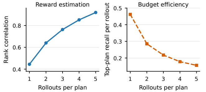
Figure 6: Plan quality estimation and top-plan discovery efficiency.
