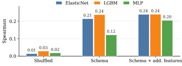
Figure 4: Schema-space reward predictability.
