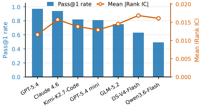
Figure 7: Effect of LLM realization models on implementation success and factor quality.
