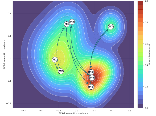
Figure 5: Semantic-space navigation across search rounds.
