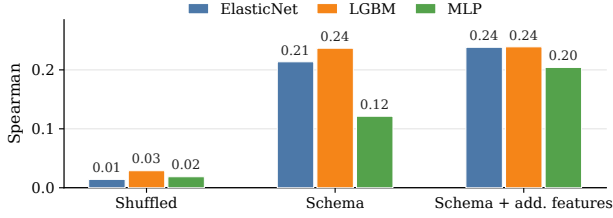
Figure 7: Reward predictability from structured schema features.
