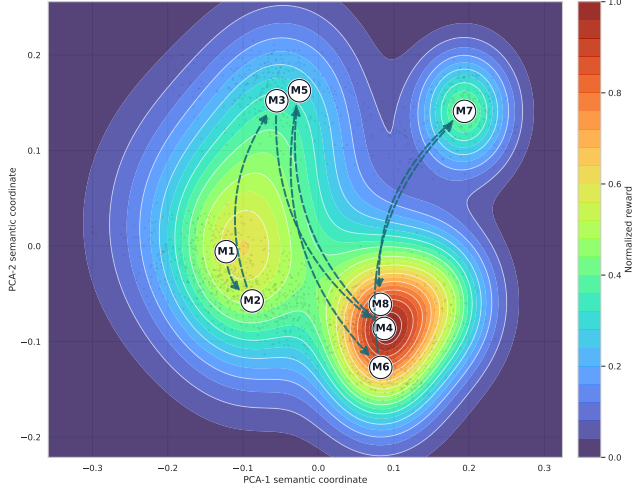
Figure 4: Semantic-space navigation across search rounds.
