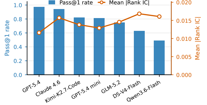
Figure 6: Effect of LLM realization models on implementation success and factor quality.
