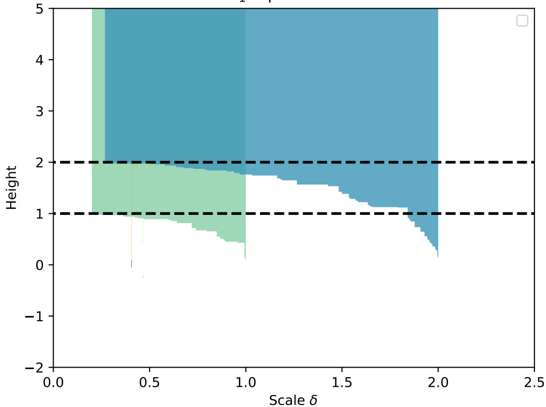
H_1 2-persistence
