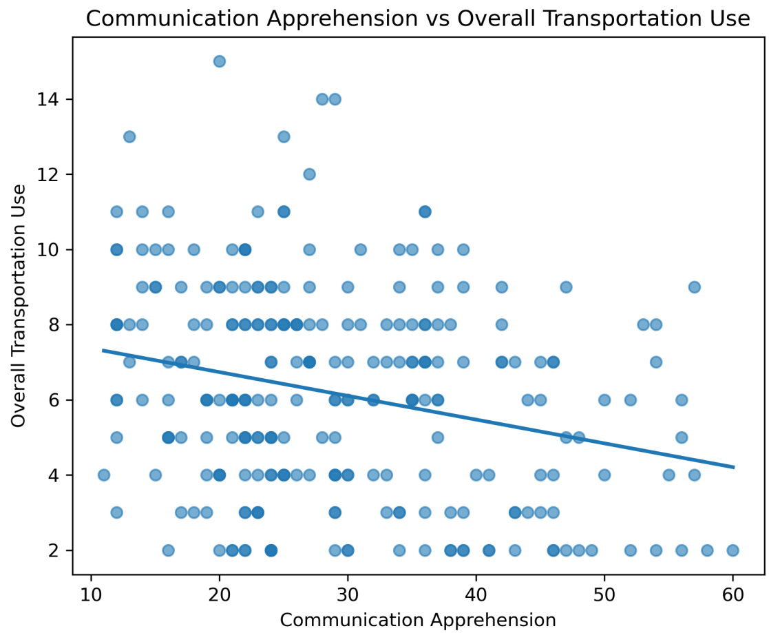
Figure 7: Communication apprehension vs. overall transportation use.
