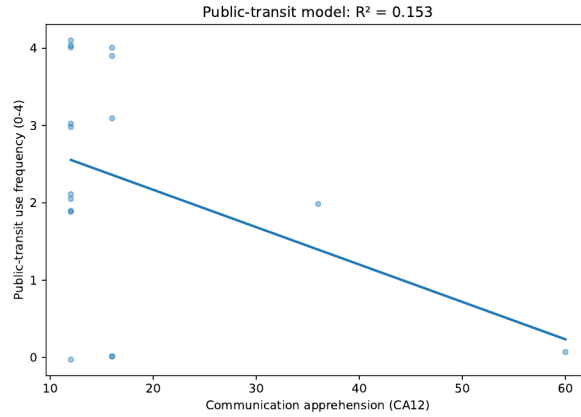
Figure 1: Public-transit use as a function of CA12.
