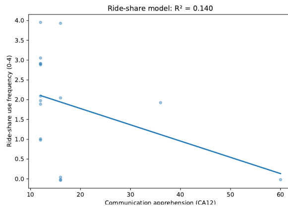
Figure 2: Ride-share use as a function of CA12.
