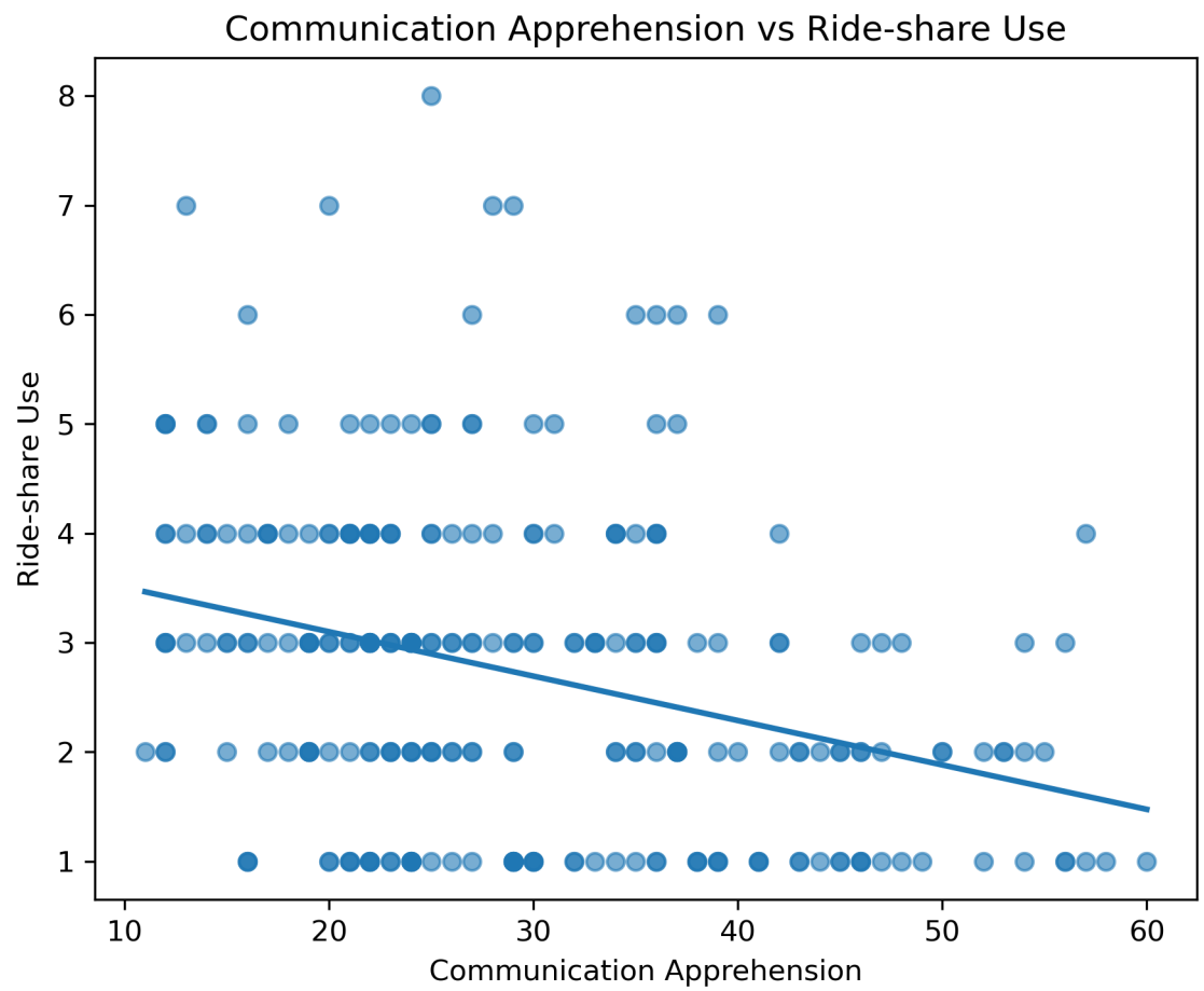
Figure 6: Communication apprehension vs. ride-share use.
