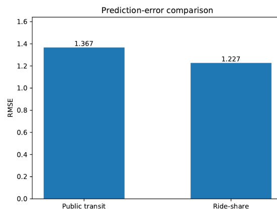
Figure 3: RMSE comparison for the public-transit and ride-share models.
