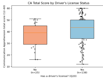
Figure 4: CA_total by driver’s-license status.
