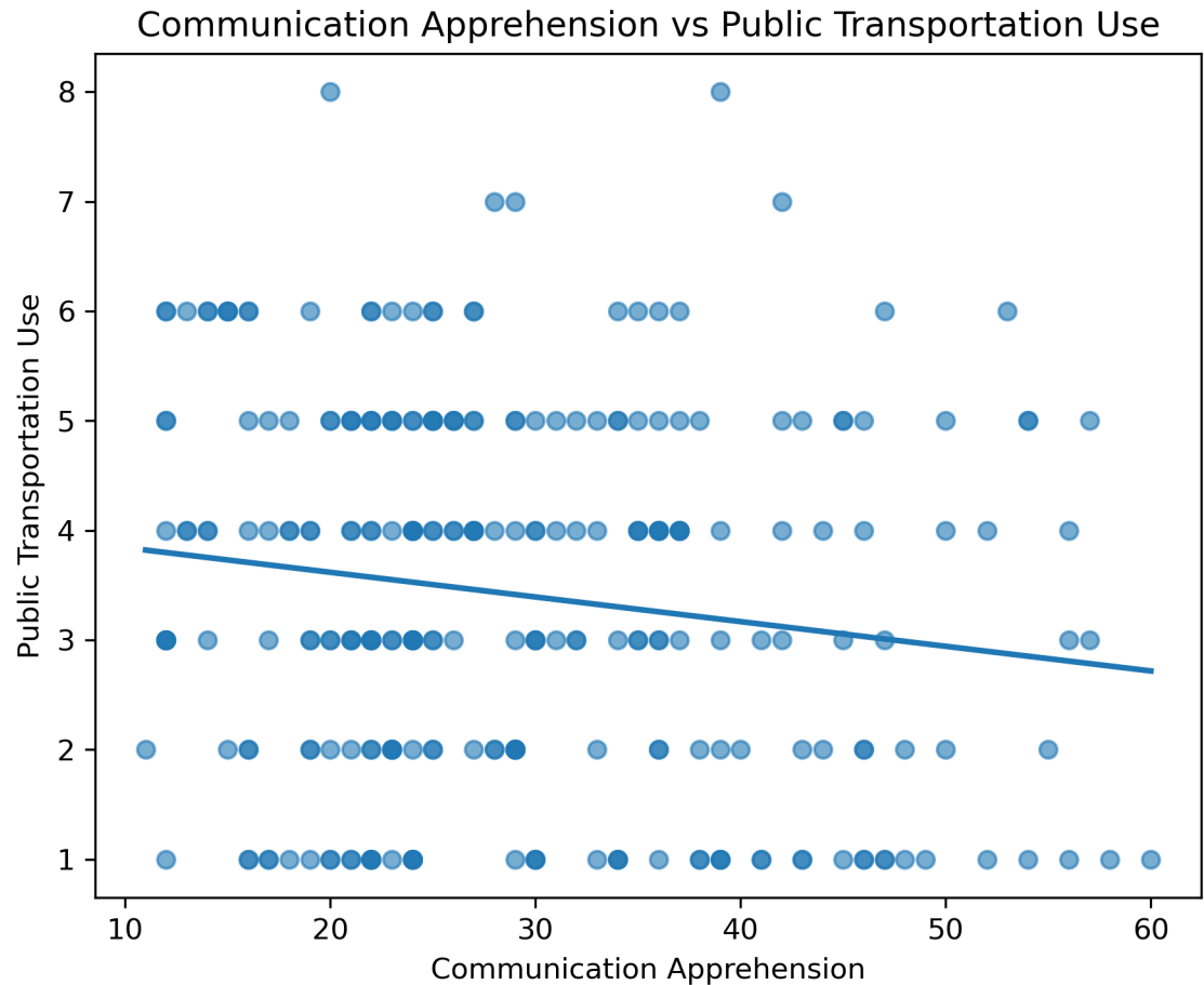
Figure 5: Communication apprehension vs. public-transportation use.
