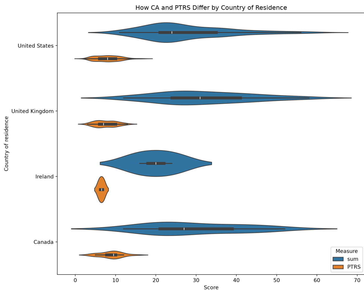
Figure 10: Communication apprehension (“sum”) and combined transportation use (“PTRS”) by country of residence, restricted to the four largest-sample countries.
