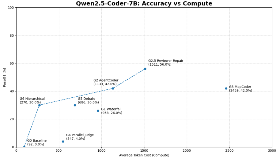
Fig. 2. Accuracy vs. Compute for Qwen2.5-Coder-7B. The Pareto frontier shifts compared to GPT-5.4 Nano, highlighting the interaction between model capability and optimal topology design.
