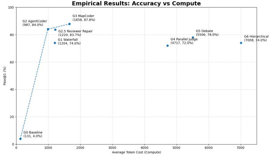
Fig. 1. Accuracy vs. Compute for GPT-5.4 Nano across graph topologies. The Pareto frontier consists of G0, G2, and G3, indicating that cyclic execution-based structures achieve the best tradeoff between accuracy and token cost.
