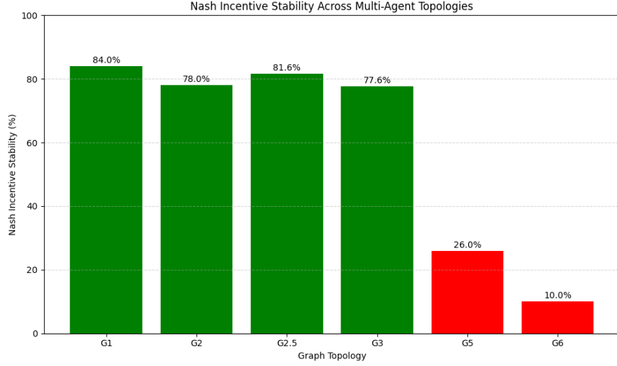
Fig. 3. Nash incentive stability across graph topologies. Loop-based structures (G1–G3) maintain high stability, while redundant parallel and hierarchical systems (G5, G6) exhibit significant instability due to free-riding incentives.
