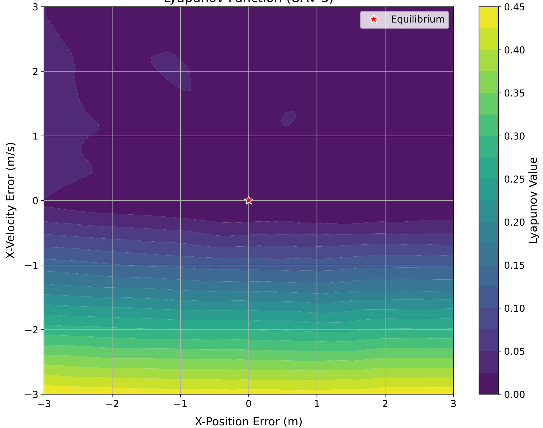
Lyapunov Function (UAV 3)
