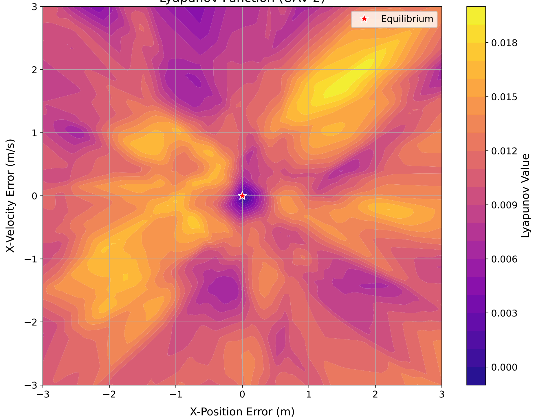
Lyapunov Function (UAV 2)
