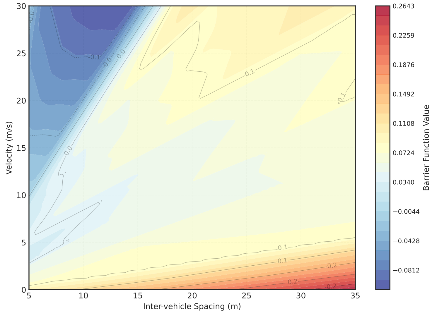
Safety Barrier Function - Vehicle 1
