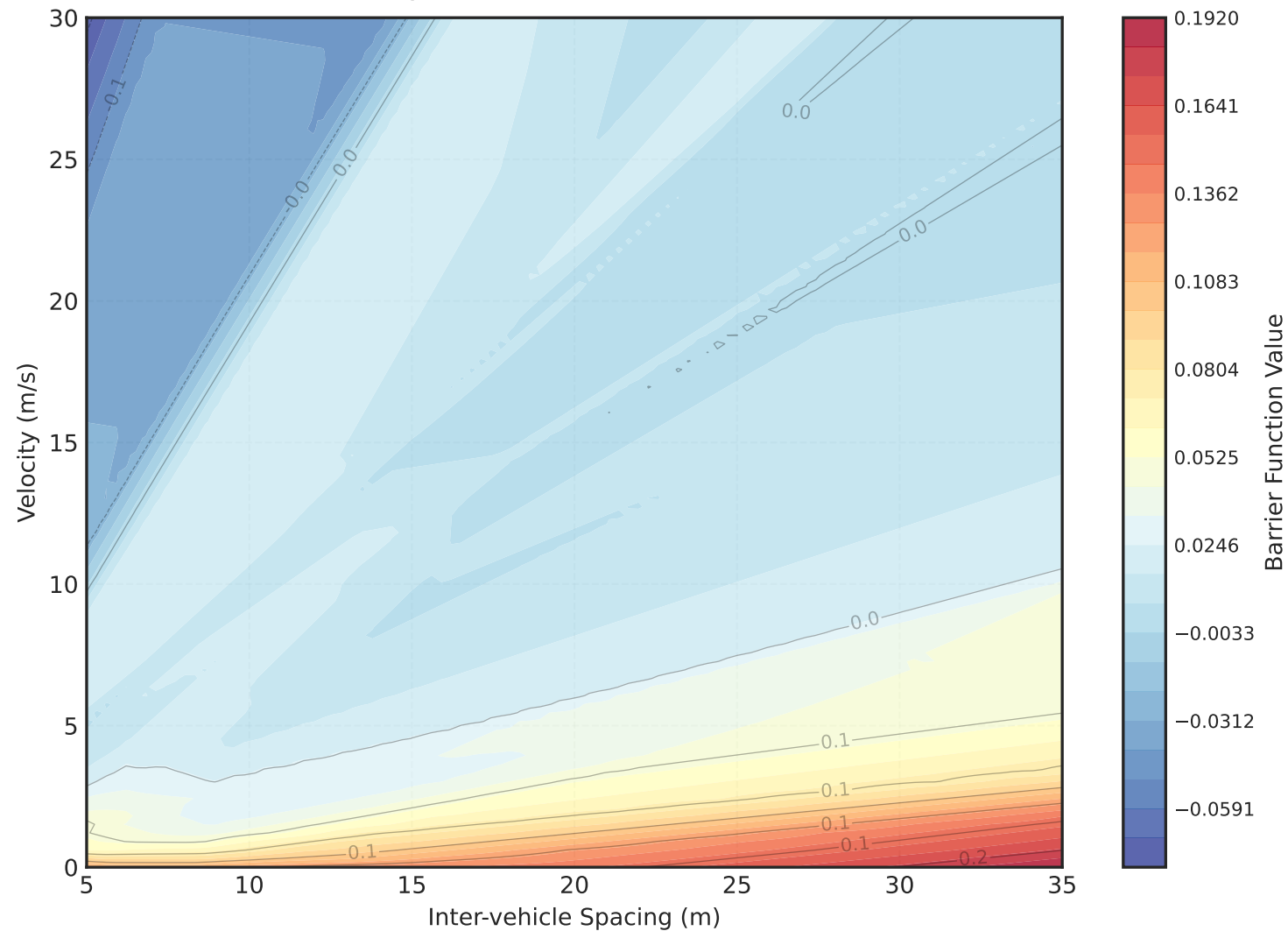
Safety Barrier Function - Vehicle 3
