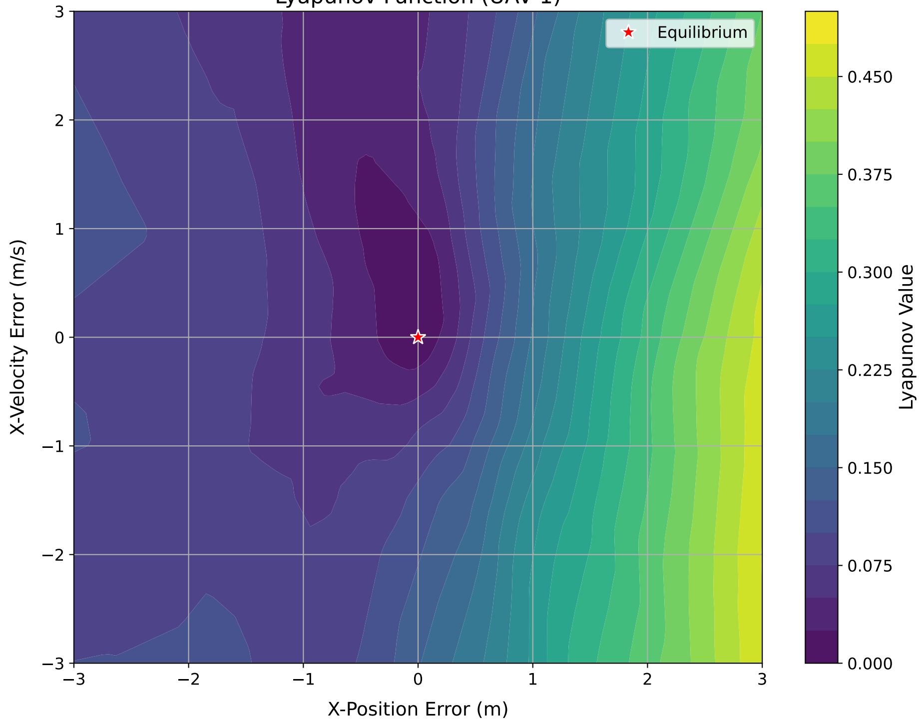
Lyapunov Function (UAV 1)
