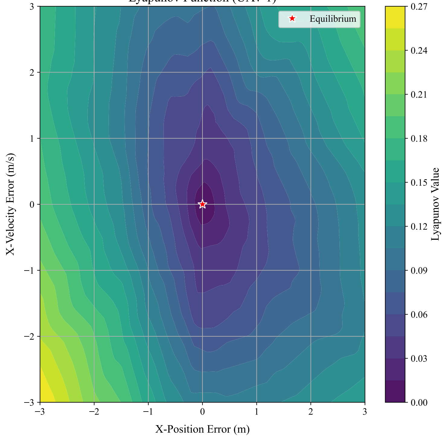
Lyapunov Function (UAV 1)
