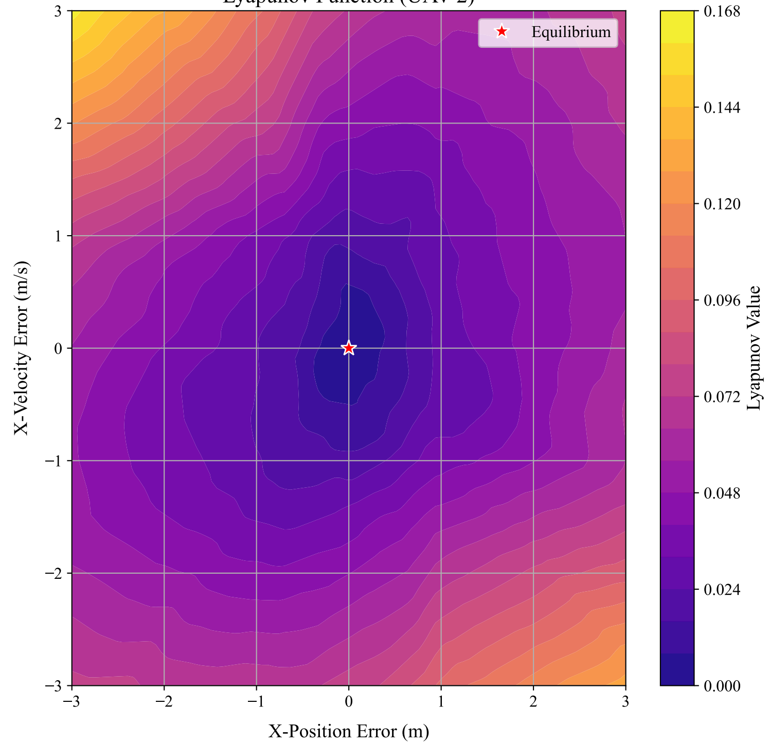
Lyapunov Function (UAV 2)
