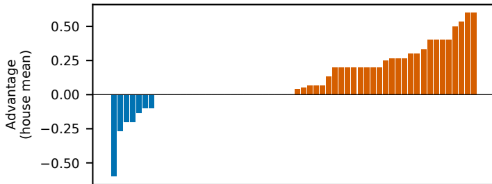
Simulator instance masks: Identity continuity 58 houses; favourable 29, unfavourable 7, zero 22
