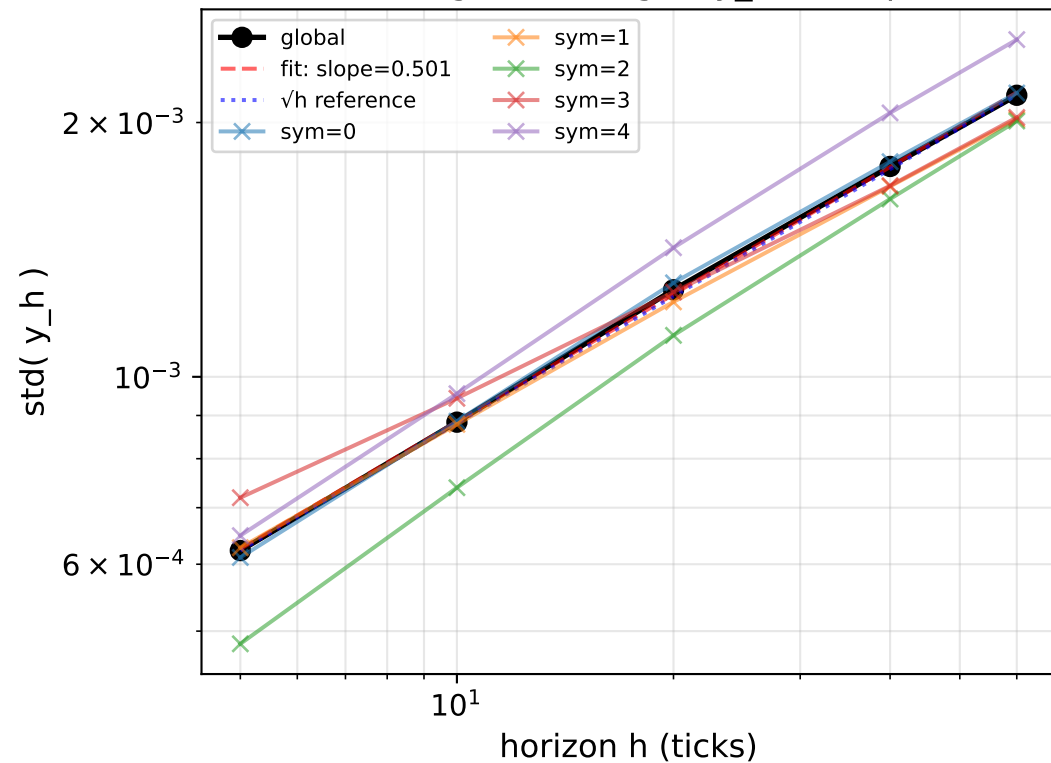
A1. Signal scaling: \sigma(y_h) \propto h^p
