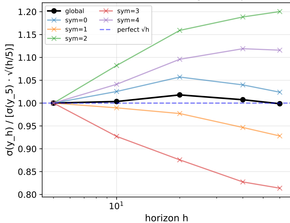
A2. Deviation from \sqrt{h} scaling (1.0 = perfect)
