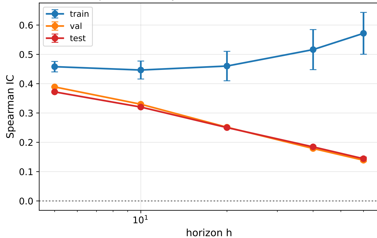
C1. Spearman IC by horizon (5 seeds, mean \pm std)
