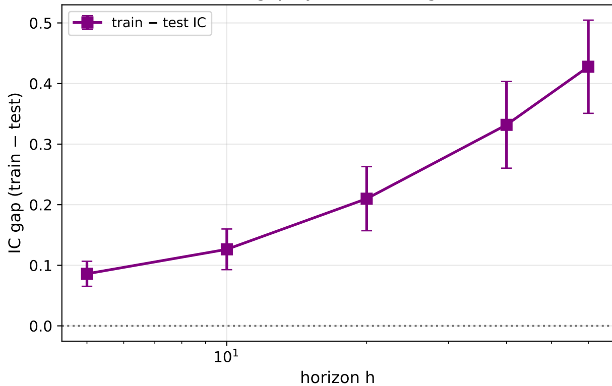
C2. Generalization gap by horizon (larger \Rightarrow worse OOD)
