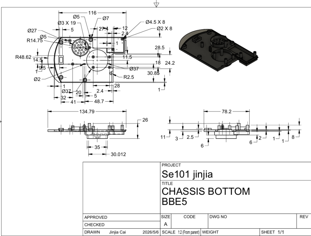
Appendix B: Tolerance Drawings
