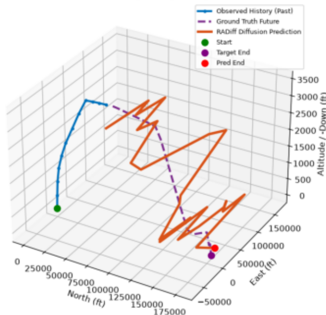
GUAM UAM Trajectory Sample #2
