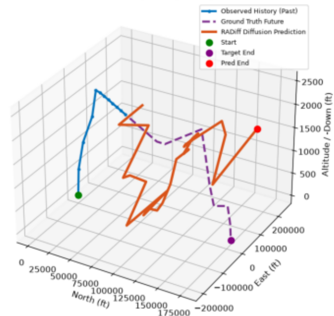
GUAM UAM Trajectory Sample #3
