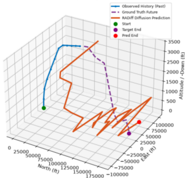
GUAM UAM Trajectory Sample #1
