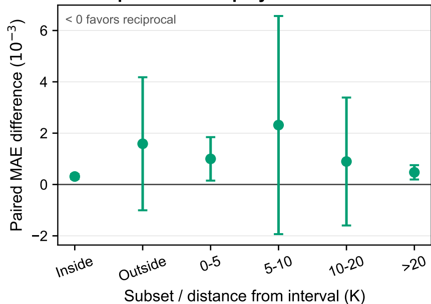
D Reciprocal minus polynomial
