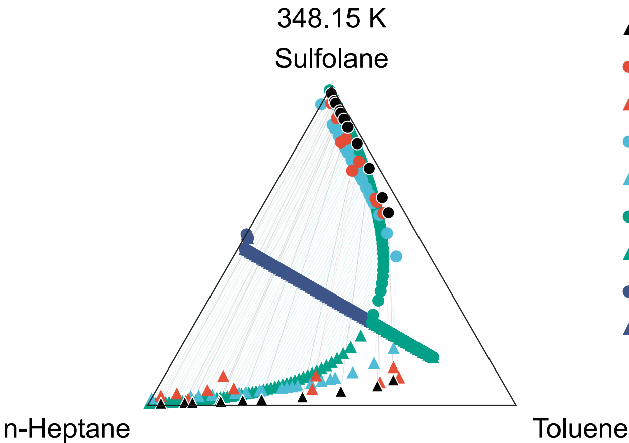
c n-Heptane + Toluene + Sulfolane
