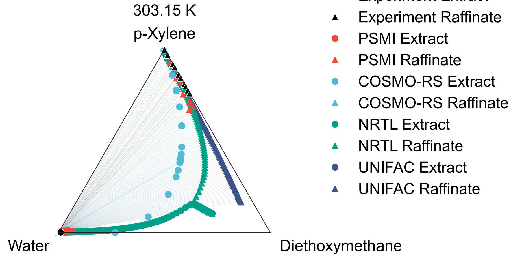
d Water + Diethoxymethane + p-Xylene
