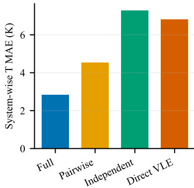
Ternary temperature
