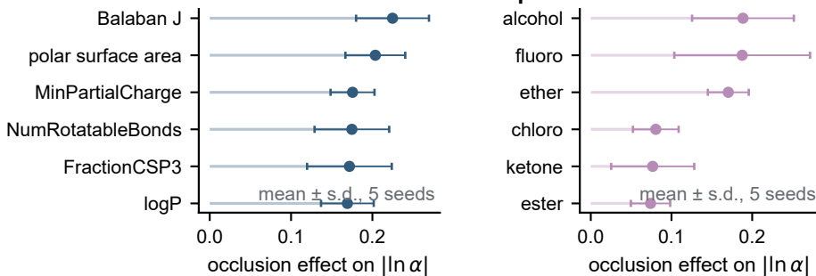
f Explicit held-out chemical case studies
