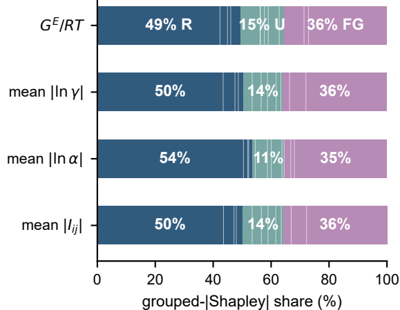
d Named chemical feature importance
