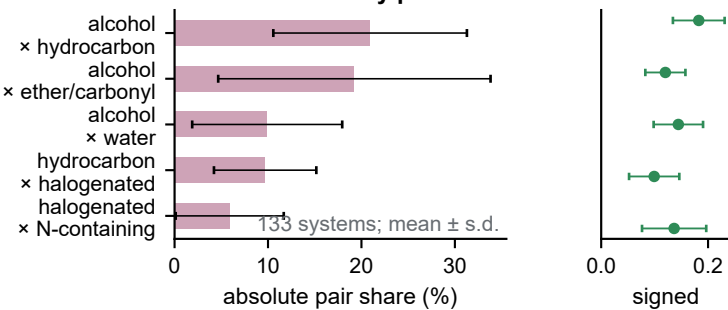
e Dominant binary pair contributions
