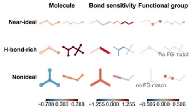
c Multilevel molecular interpretation of mean |\ln \alpha|
