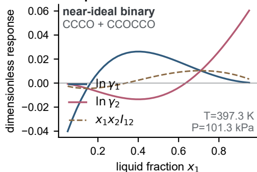
f Explicit held-out chemical case studies
