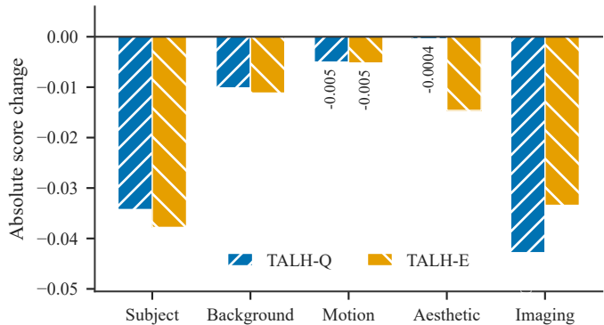
(b) VBench change from Native-HR
