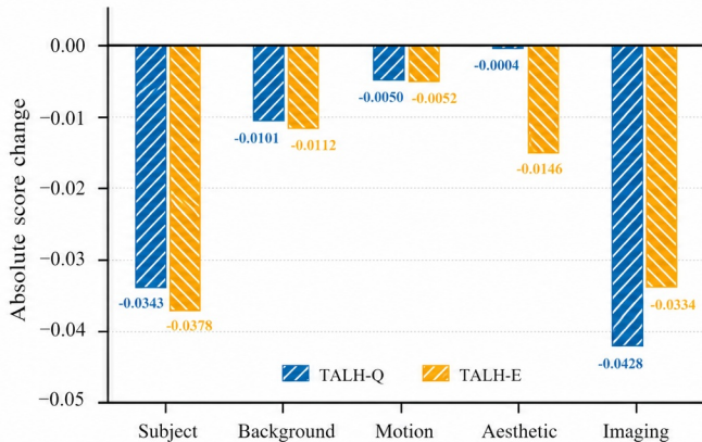
(b) VBench change from Native-HR
