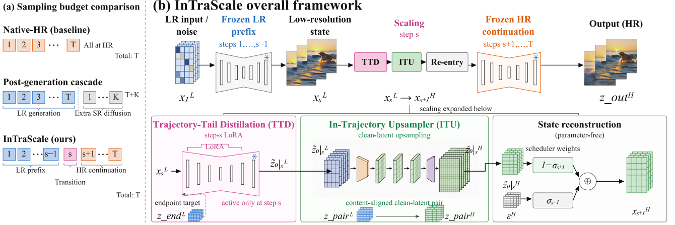
Figure 2: Sampling budget and overall framework of InTraScale. (a) Native-HR executes all T steps at target resolution, whereas a post-generation cascade appends additional K steps. (b) At step s , TTD distills the omitted low-resolution trajectory tail into an endpoint-calibrated clean prediction. ITU, trained on low- and target-resolution clean-latent pairs, lifts this prediction to the target-resolution latent space. HR and LR denote target- (720p) and low-resolution (368p) sampling.
