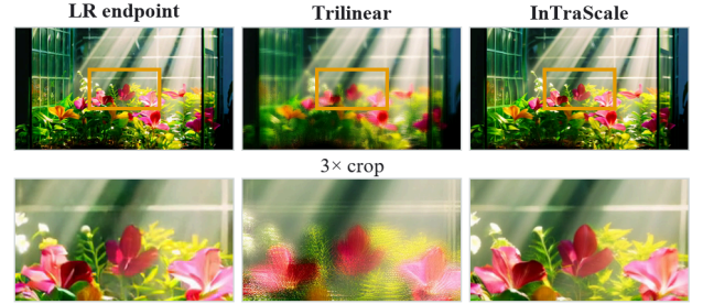
Figure 3: Trilinear interpolation under a late resolution transition. The columns show the completed LR endpoint after 50 low-resolution steps, Trilinear@40, and InTraScale@40; the bottom row shows the corresponding 3\times crops.
