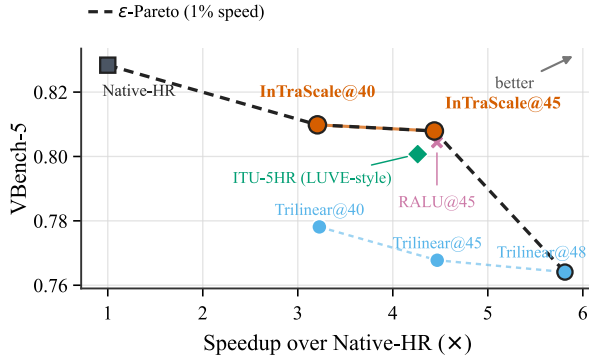
Figure 5: 50-step quality–efficiency Pareto frontier.
