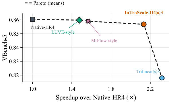
Figure 6: 4-step quality-efficiency Pareto frontier.
