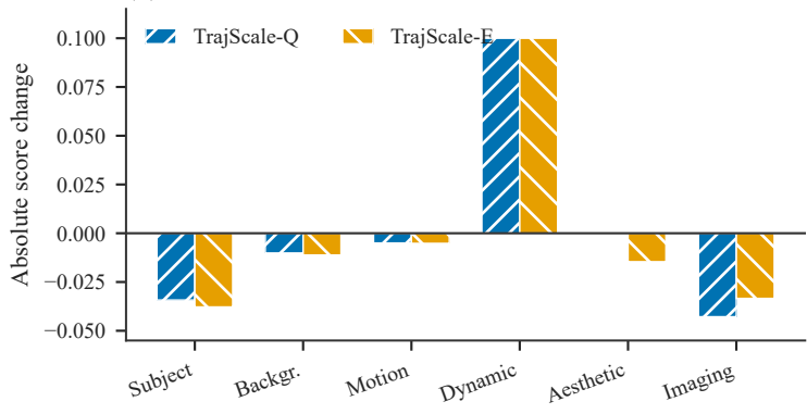
(b) VBench dimensions vs. Native-HR
