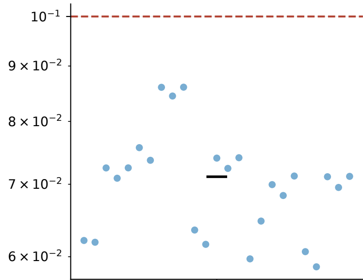
Output coefficient L1 error
