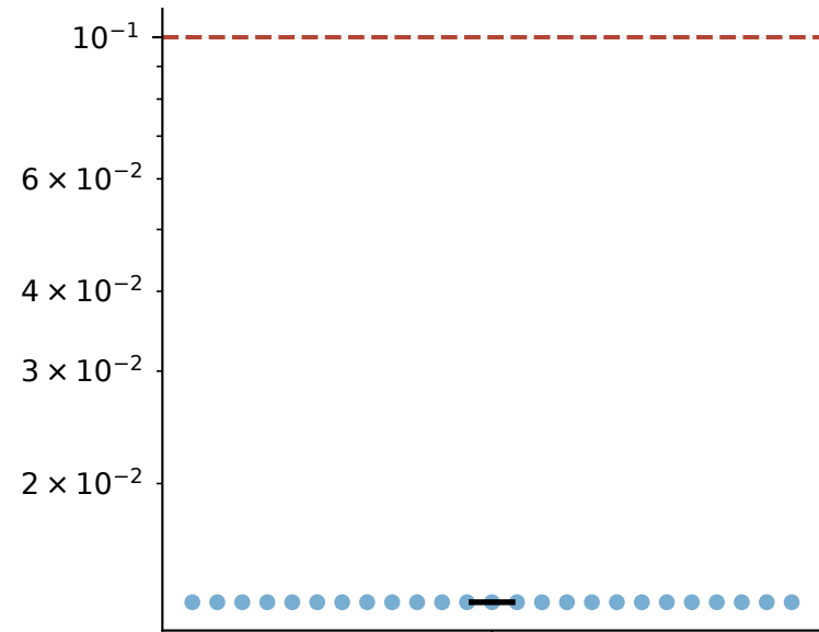
First-layer operator error
