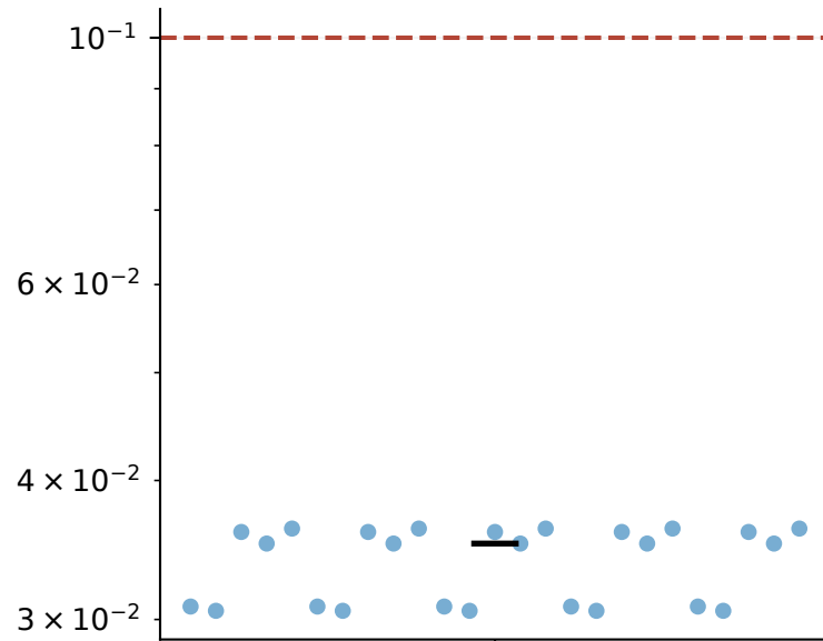
Second-layer operator error
