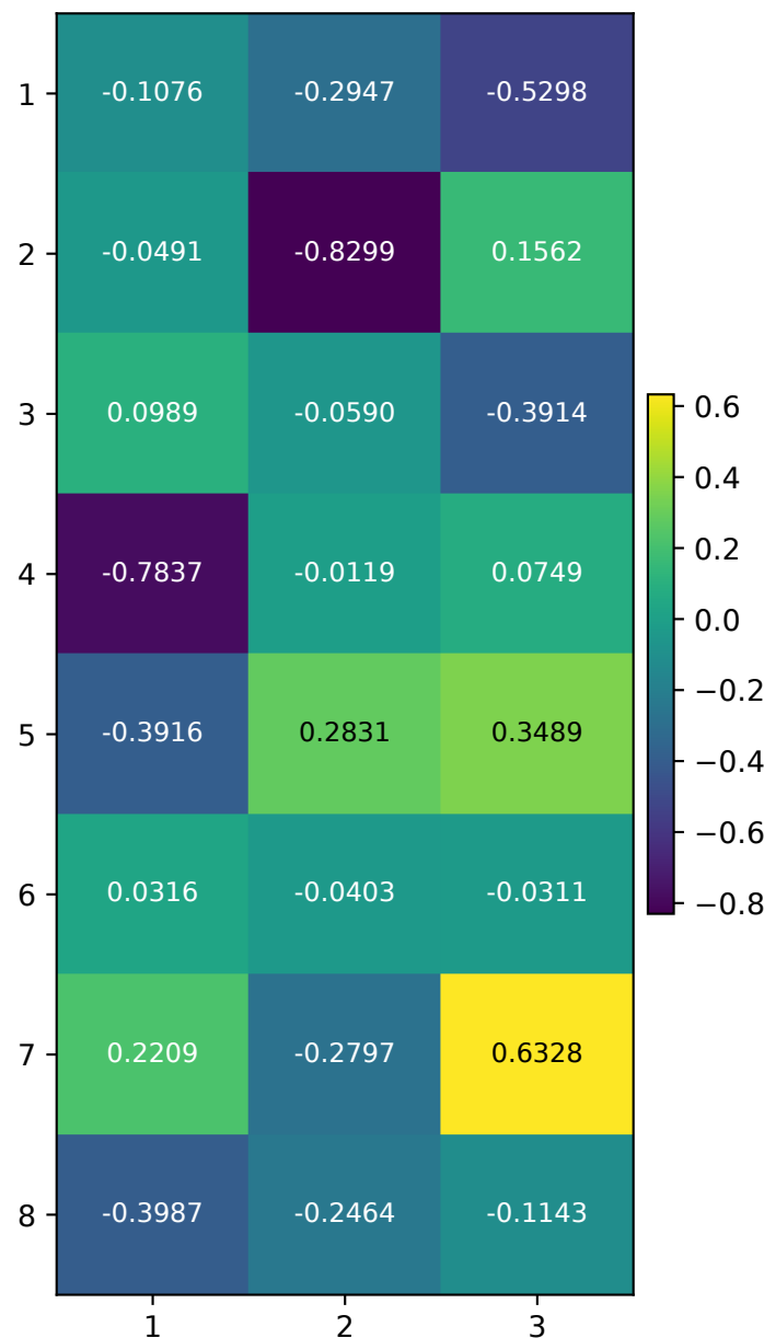
W2: Recovered
