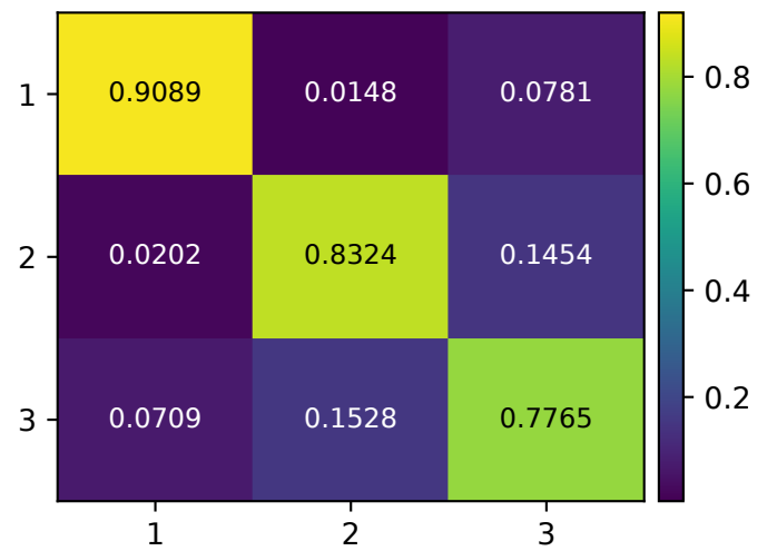
a: Recovered
