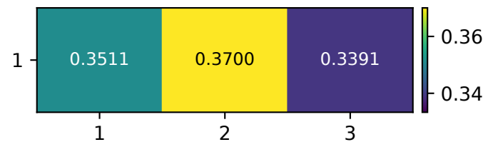
a: Recovered
