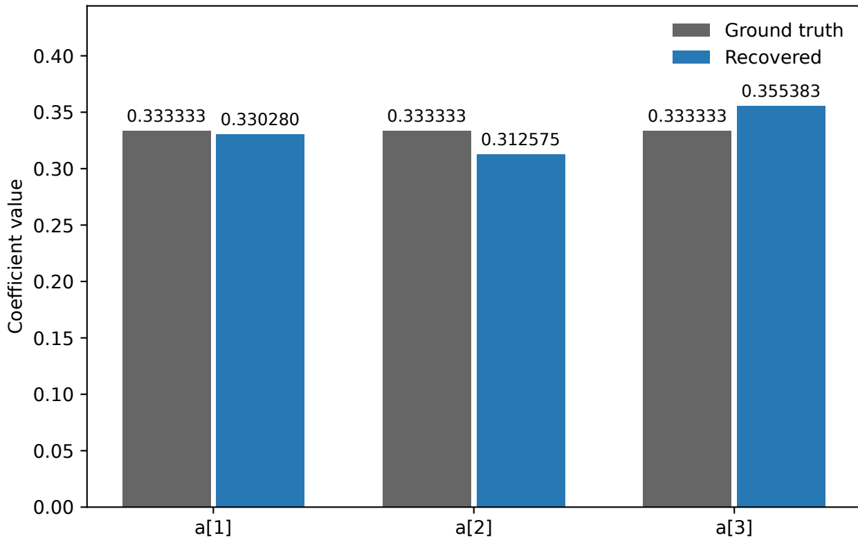
Experiment 1 (k=8): output coefficients
