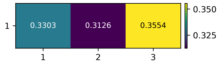
a: Recovered
