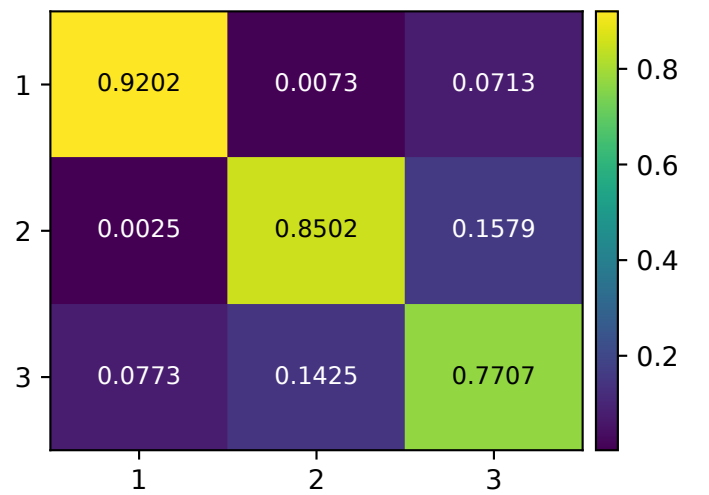
a: Recovered
