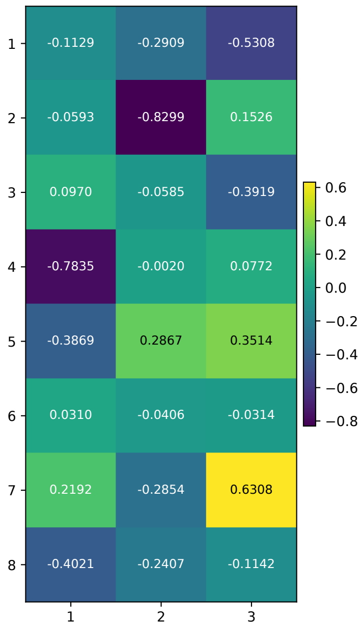
W2: Recovered
