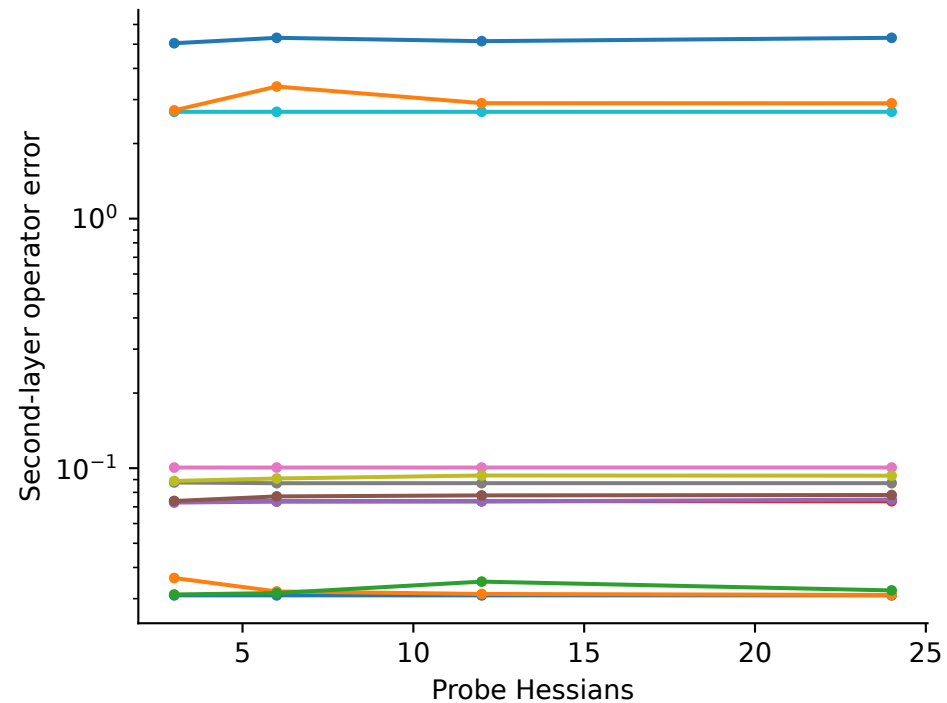
More probes and smaller residuals do not guarantee better recovery
