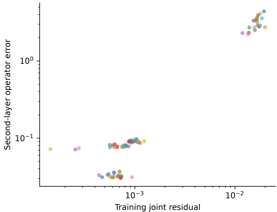
More probes and smaller residuals do not guarantee better recovery
