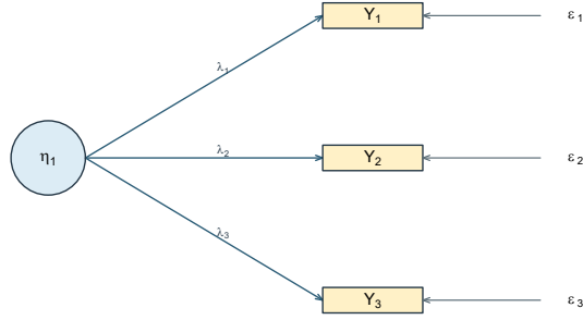
Figure 1: A latent variable with three indicators. Rectangles are recorded variables, the circle is a variable introduced by the model, and single-headed arrows denote loading relations.
