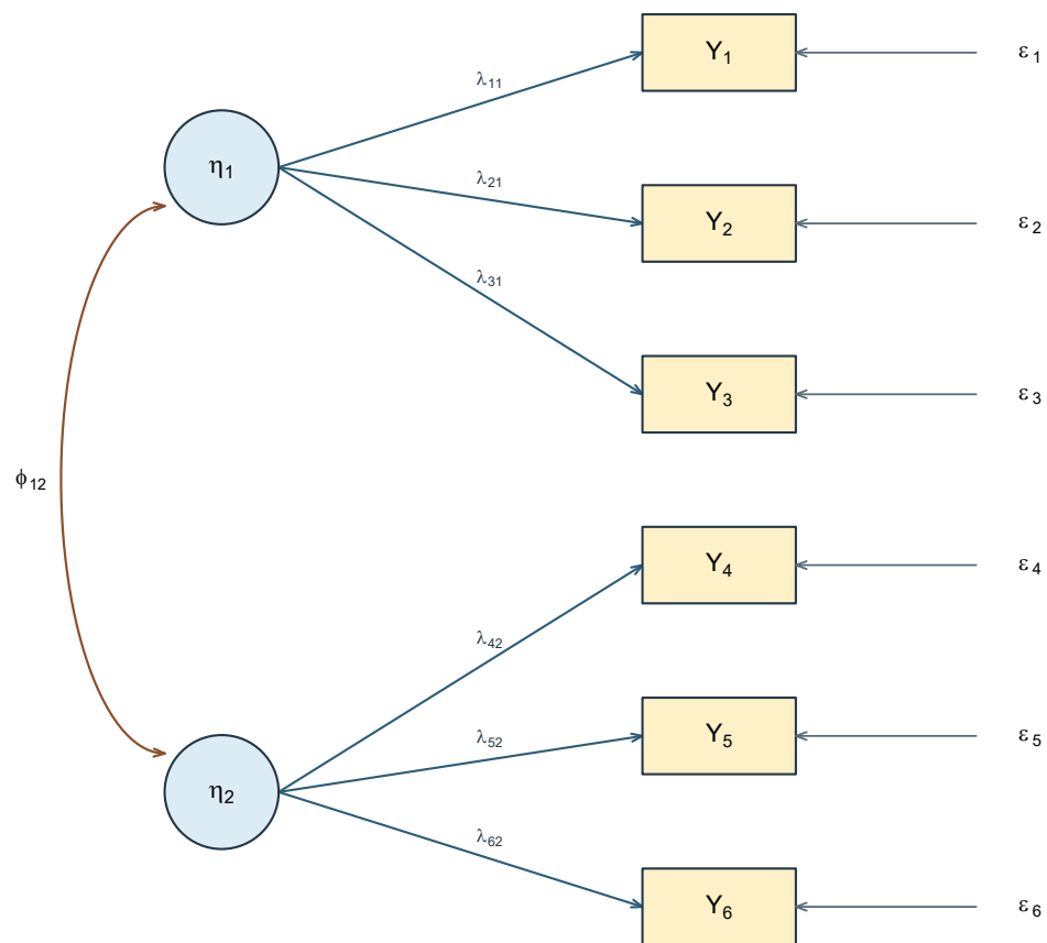
Figure 3: The same system restricted to a simple structure. Each indicator has one loading and one residual; the six cross-loadings are fixed at zero.
