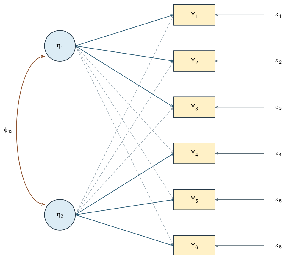
Figure 2: The two-factor, six-indicator system with every loading present. Single-headed arrows denote loading relations; the double-headed arrow denotes the factor covariance.
