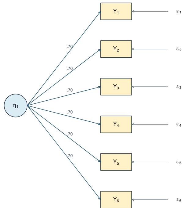
Figure 4: The one-factor model that reproduces the first record. Every loading is .70 .
